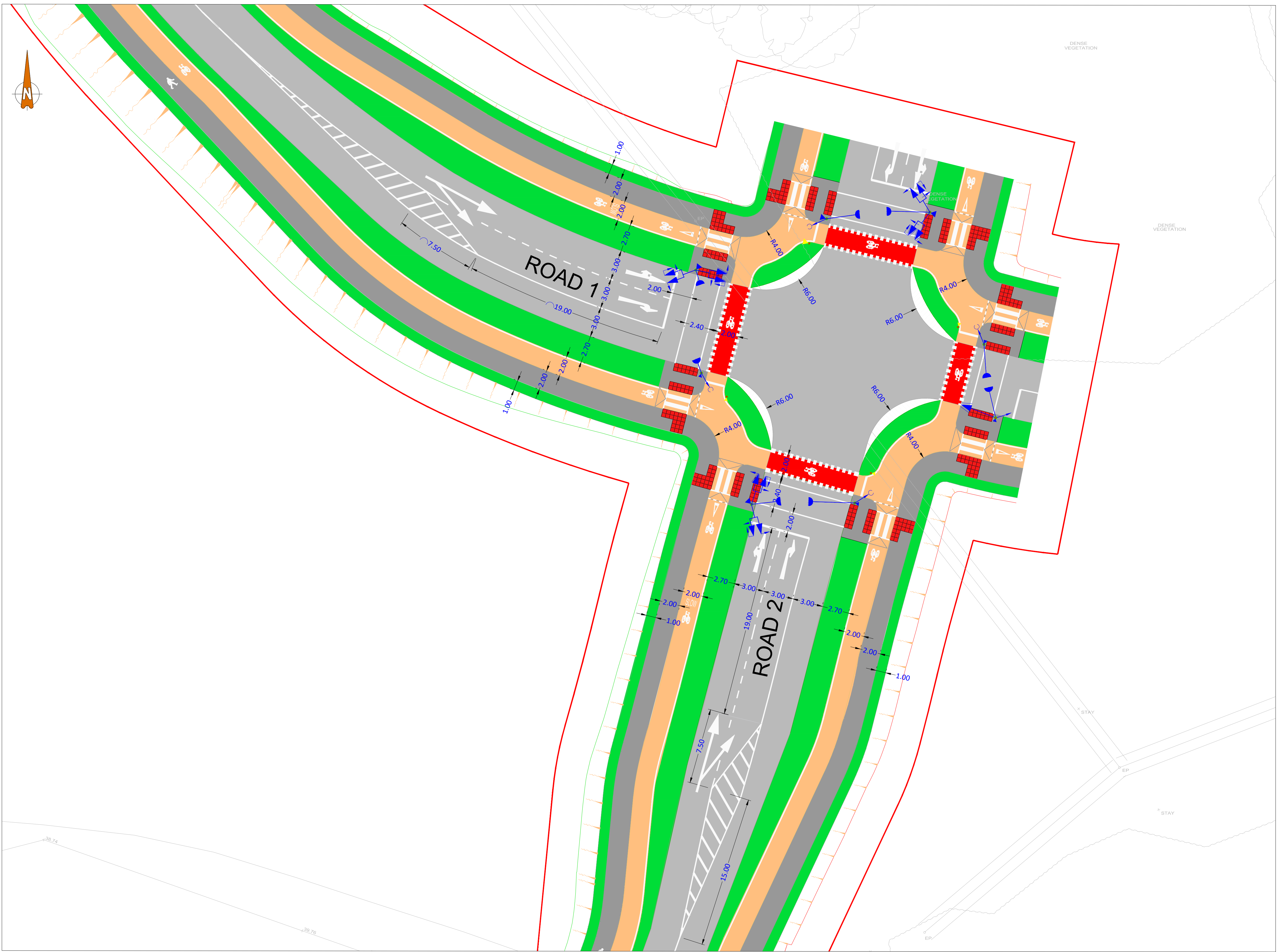
JUNCTION LAYOUT SCALE 1:200
